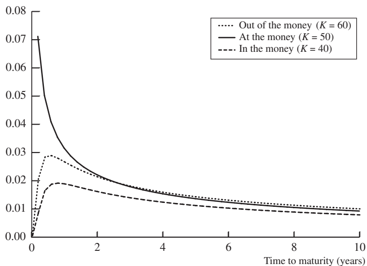
Figure 17.10 Variation of gamma with time to maturity for a stock option ( S_0 = 50 , r = 0 , \sigma = 20\% )
