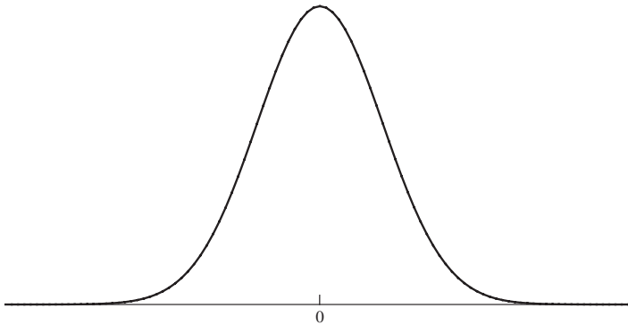
Figure 13.2 A normal distribution
