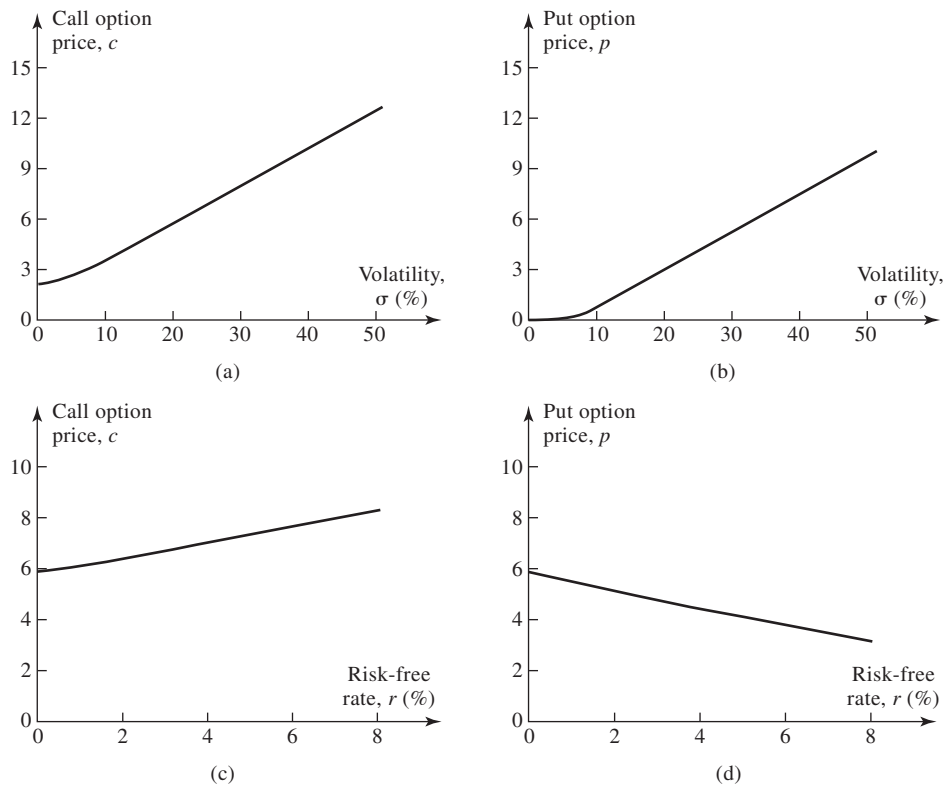
Figure 10.2 Effect of changes in volatility and risk-free interest rate on option prices when S_0 = 50 , K = 50 , r = 5\% , \sigma = 30\% , and T = 1
